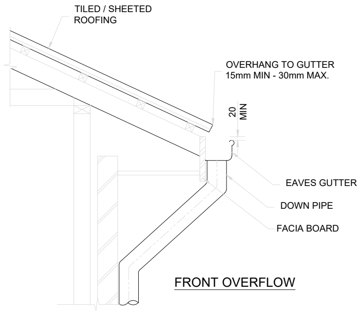
TYPICAL EAVES GUTTER DETAIL 1:20
